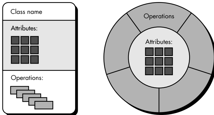
FIGURE 20.4 An alternative representation of an object-oriented class
