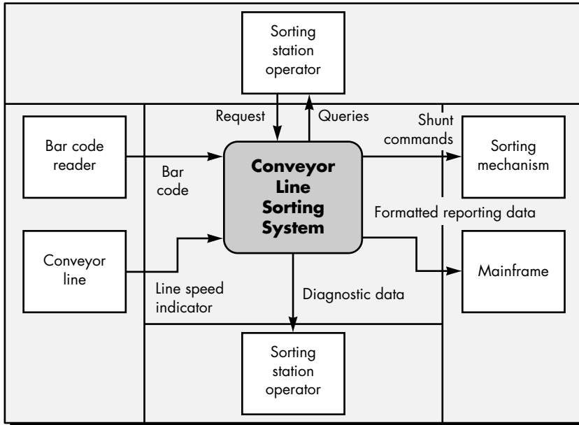
FIGURE 10.6 System context diagram for CLSS (extended)
