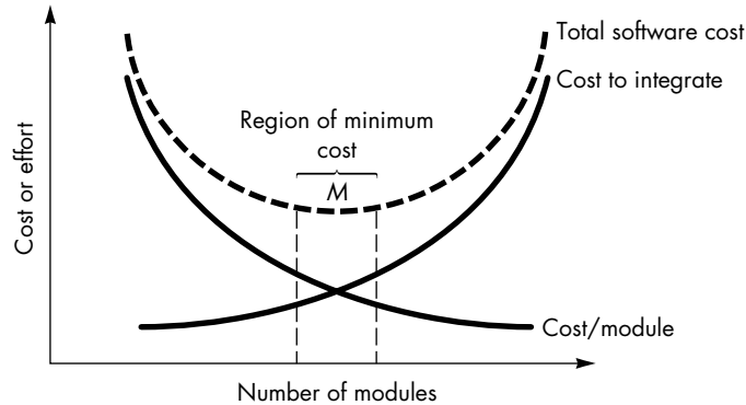
FIGURE 13.2 Modularity and software cost
